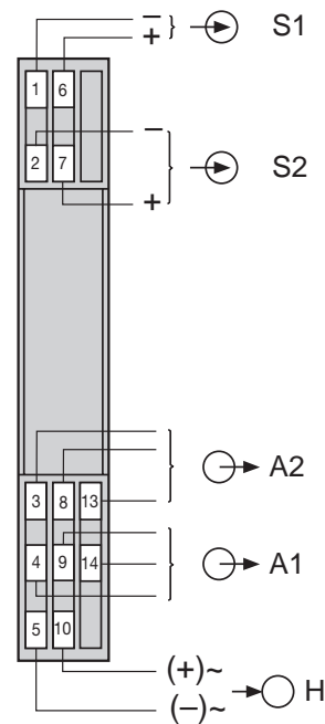
Fig. 10. Terminal allocation
